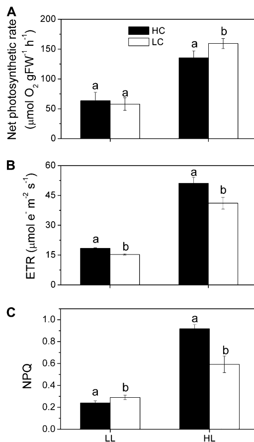
Figure 2. The net photosynthetic rate (A), ETR (B), and NPQ (C) of U. prolifera plants grown for 2 months at ambient (LC; 390 μatm) and elevated (HC; 1,000 μatm) CO 2 levels measured at growth light (LL; 100 μmol m -2 s -1 ) and high light (HL; 600 μmol m -2 s -1 ). The reaction medium (sterilized seawater) was equilibrated with the ambient or elevated CO 2 air before use. FW, Fresh weight.
