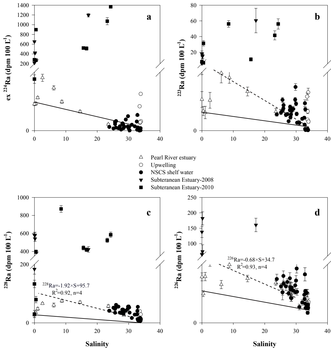
Fig. 6. Plots of (a) ex\ ^{224}\text{Ra} (excess ^{224}\text{Ra} , corrected for the ingrowth from ^{228}\text{Th} ), (b) ^{223}\text{Ra} , (c) ^{228}\text{Ra} , and (d) ^{226}\text{Ra} versus salinity in the Pearl River estuary, northern South China Sea (NSCS) shelf waters and NSCS subterranean estuary. Solid lines represent the conservative mixing line between the freshwater end-member of the Pearl River and offshore surface seawater. Dotted lines denote conservative mixing after the Ra peak with salinity > 9 in the Pearl River estuary. The linear regression equations shown in panels c and d are based on the ^{228}\text{Ra} and ^{226}\text{Ra} vs salinity plots at salinity > 9 .
